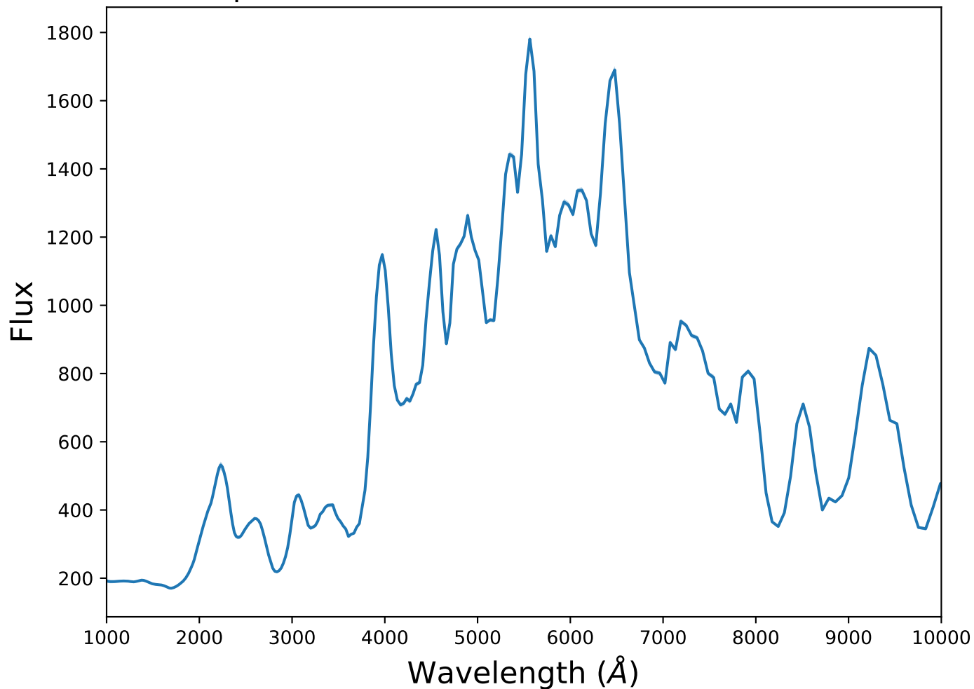
Spectrum 9 for transient SNIax at z=0.28
